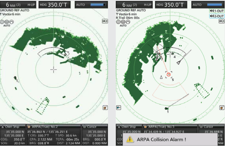
Simplified ARPA Alarm example
